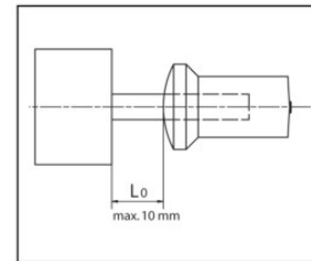
minimum bore size for wheel brushes according to DIN EN 1083
